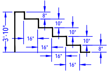
ENTRY STEP DETAIL (After Concrete & Liner) N.T.S.
