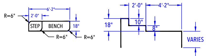
DEEP END BENCH & STEP OUT DETAIL
