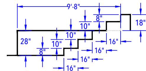
SUN DECK & ENTRY STEP DETAIL (After Concrete & Liner)
