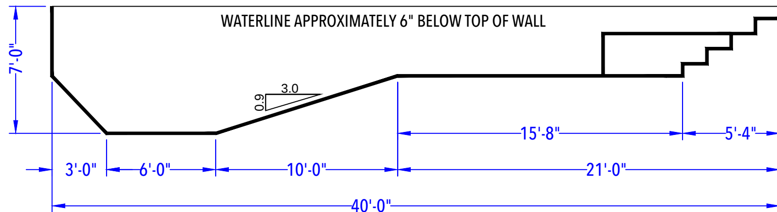
DEPTH DETAIL
