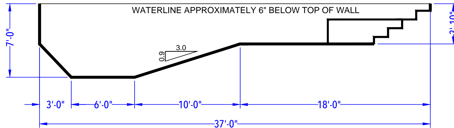
DEPTH DETAIL
