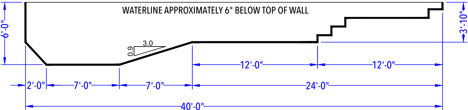
DEPTH DETAIL
