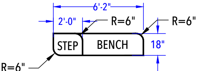
SUN DECK & ENTRY STEP DETAIL (After Concrete & Liner)
