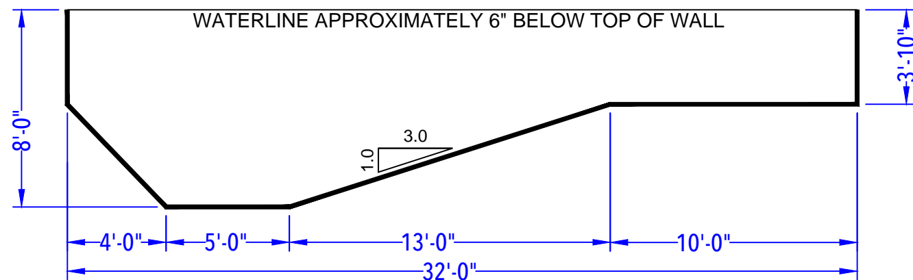
DEPTH DETAIL
