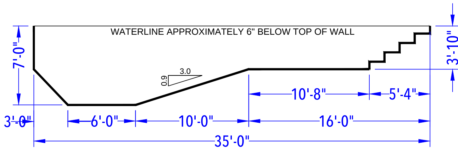
DEPTH DETAIL
