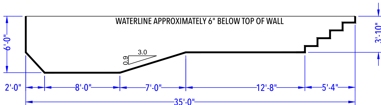
DEPTH DETAIL
