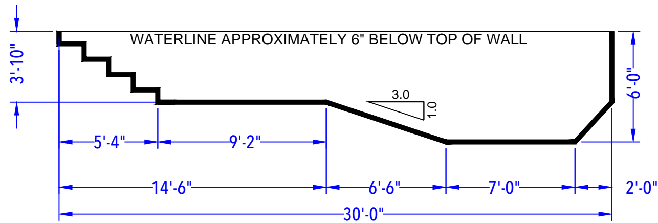
DEPTH DETAIL
