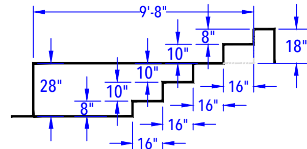
SUN DECK & ENTRY STEP DETAIL
