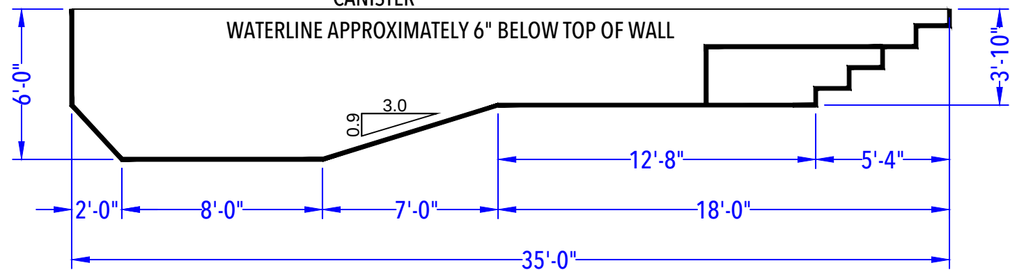
DEPTH DETAIL
