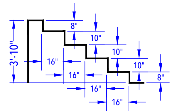
ENTRY STEP DETAIL (After Concrete & Liner) N.T.S.
