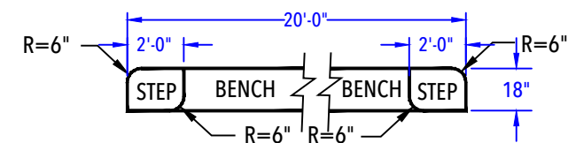
SUN DECK & ENTRY STEP DETAIL (After Concrete & Liner)
