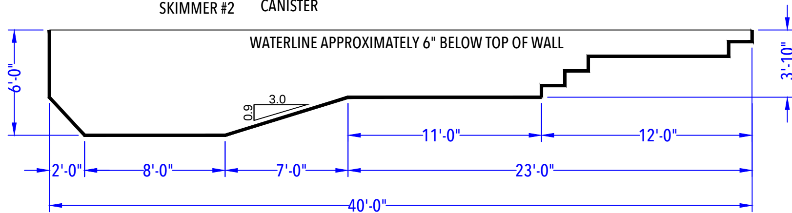
DEPTH DETAIL
