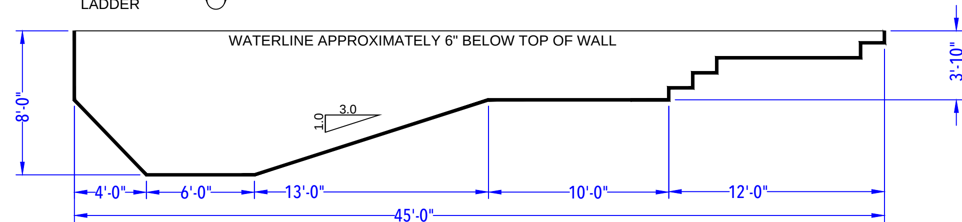
DEPTH DETAIL
