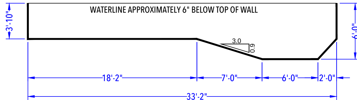
DEPTH DETAIL
