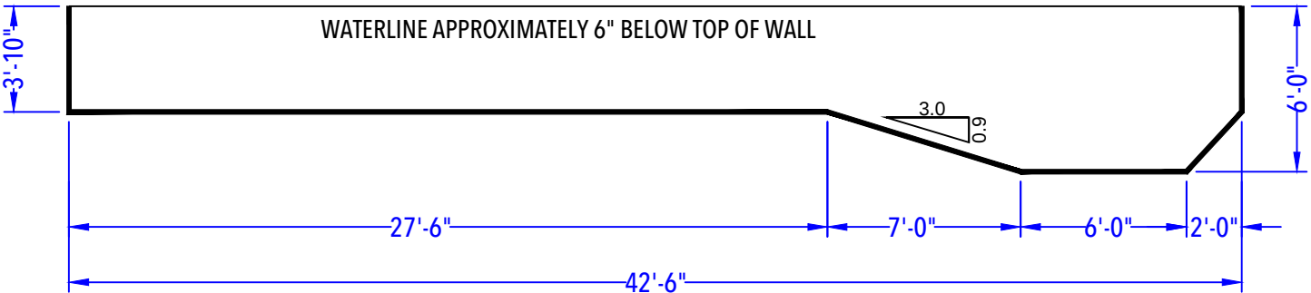
DEPTH DETAIL
