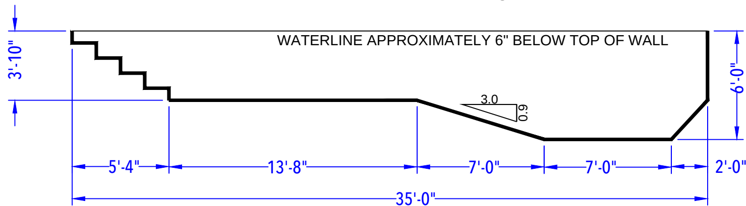
DEPTH DETAIL
