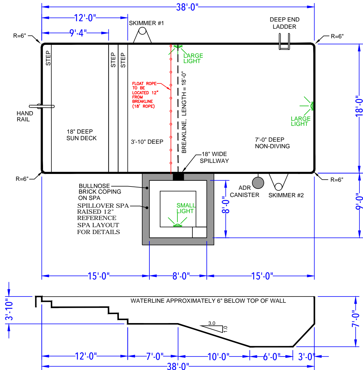
DEPTH DETAIL
