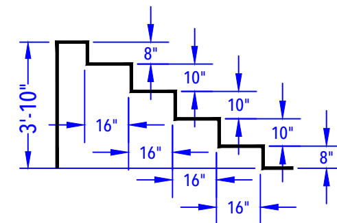
STEP DETAIL (After Bottom & Liner) N.T.S.
