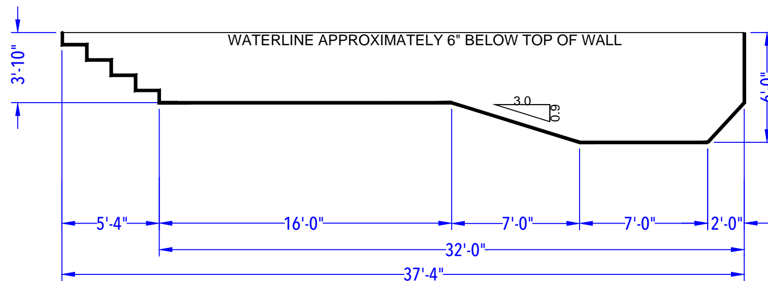
DEPTH DETAIL
