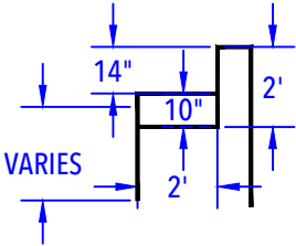
DEEP END BENCH & STEP OUT DETAIL (After Concrete & Liner) N.T.S.
