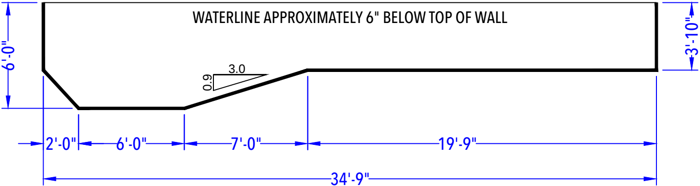
DEPTH DETAIL
