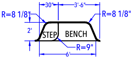
ENTRY STEP DETAIL (After Concrete & Liner) N.T.S.
