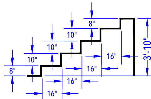
ENTRY STEP DETAIL (After Concrete & Liner) N.T.S.
