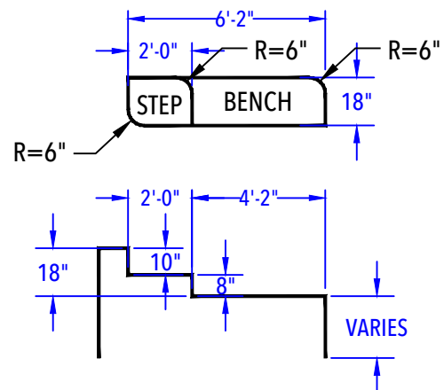
DEEP END BENCH & STEP OUT DETAIL (After Concrete & Liner) N.T.S.
