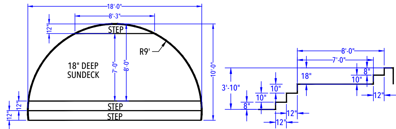
SUN DECK & ENTRY STEP DETAIL (After Concrete & Liner) N.T.S.
