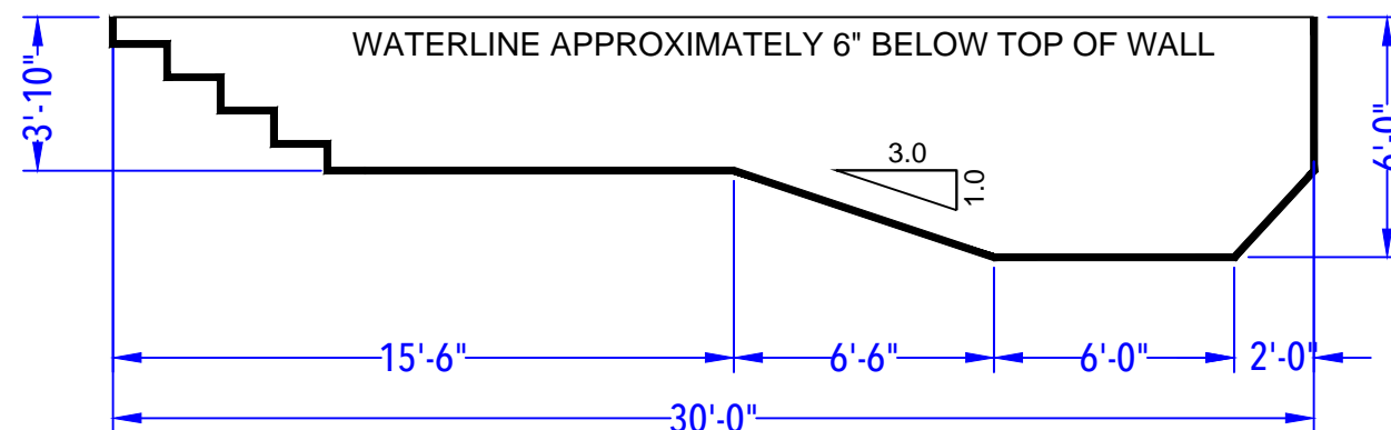
DEPTH DETAIL
