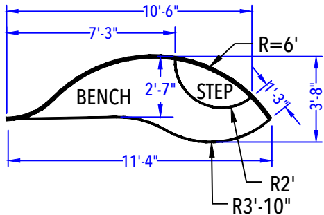
DEEP END BENCH & STEP OUT DETAIL (After Concrete & Liner) N.T.S.
