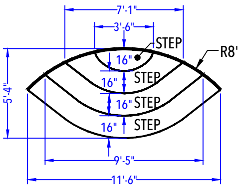
ENTRY STEP DETAIL (After Concrete & Liner) N.T.S.
