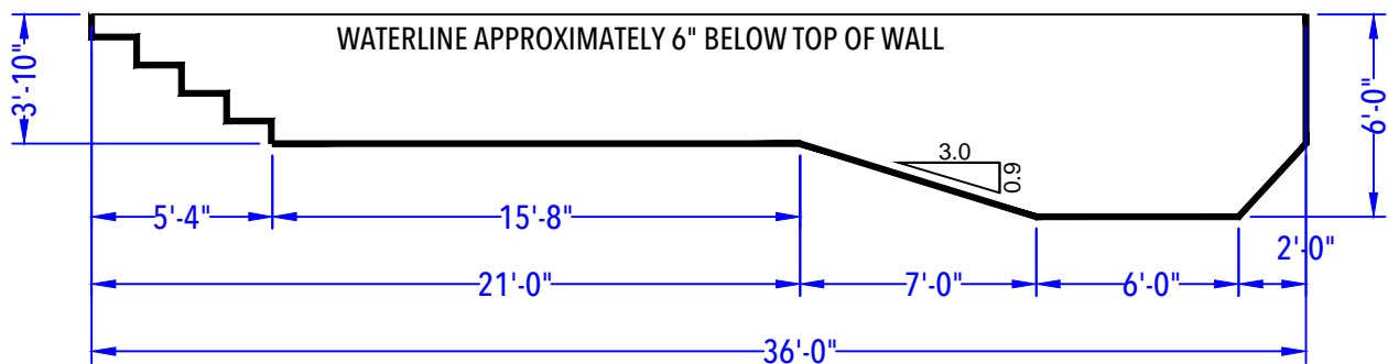
DEPTH DETAIL
