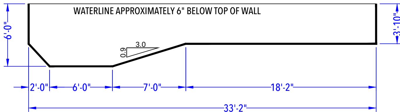
DEPTH DETAIL
