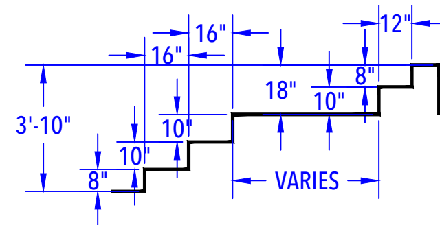
SUN DECK & ENTRY STEP DETAIL (After Concrete & Liner) N.T.S.
