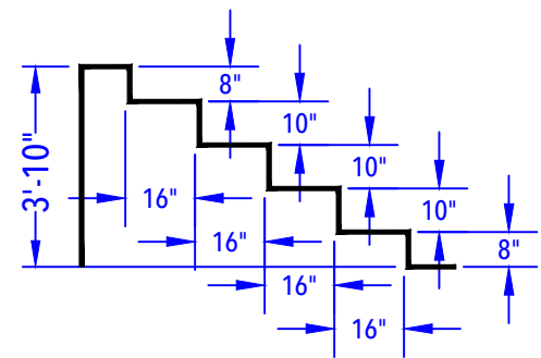
ENTRY STEP DETAIL (After Concrete & Liner) N.T.S.
