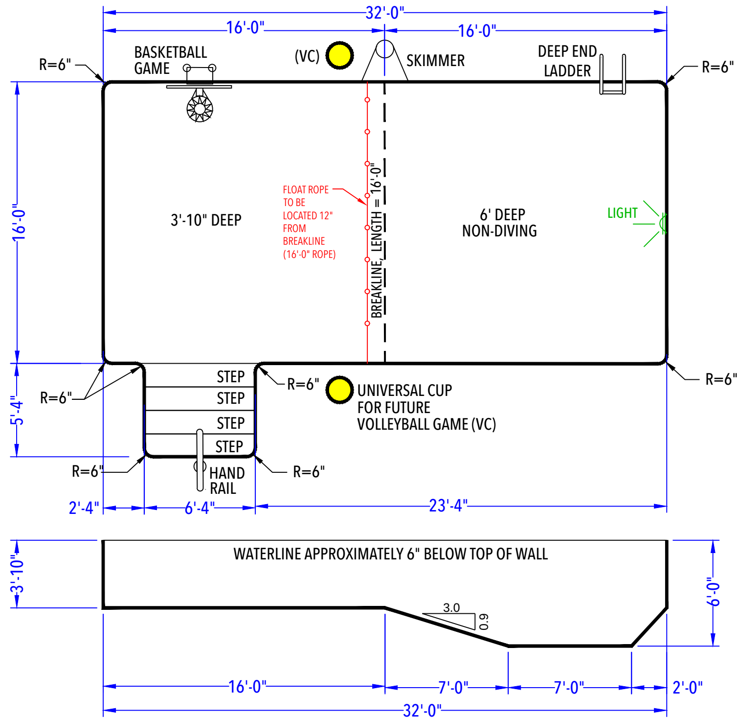
DEPTH DETAIL
