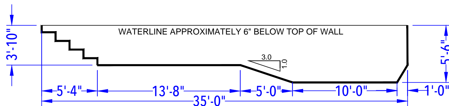
DEPTH DETAIL
