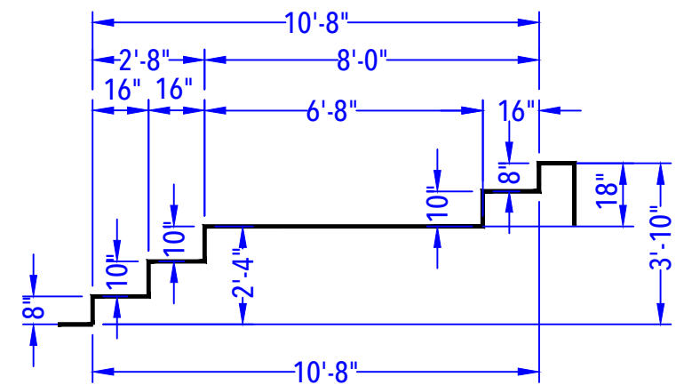
SUN DECK & ENTRY STEP DETAIL (After Concrete & Liner) N.T.S.
