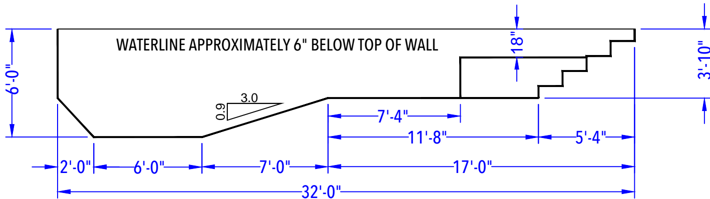
DEPTH DETAIL
