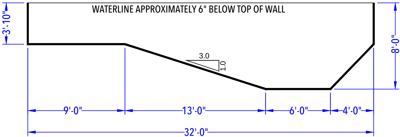
DEPTH DETAIL
