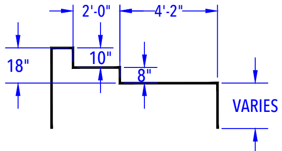
DEEP END BENCH & STEP OUT DETAIL (After Concrete & Liner) N.T.S.
