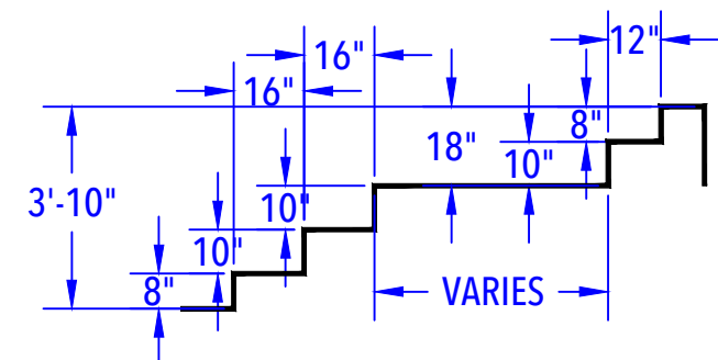
SUN DECK & STEP DETAIL (After Bottom & Liner) N.T.S.
