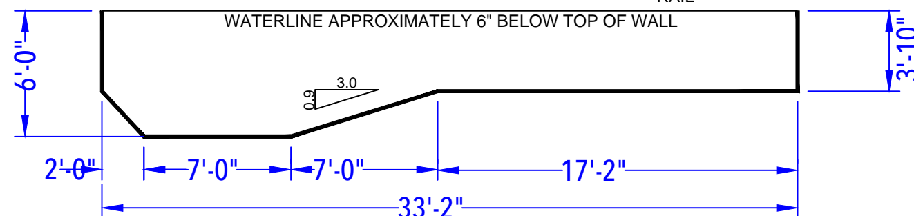
DEPTH DETAIL
