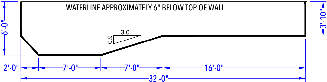
DEPTH DETAIL
