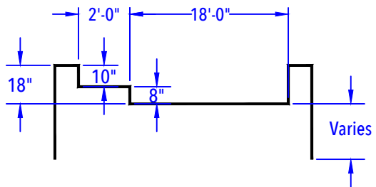
OFFSET BENCH & STEP OUT DETAIL (After Concrete & Liner) N.T.S.
