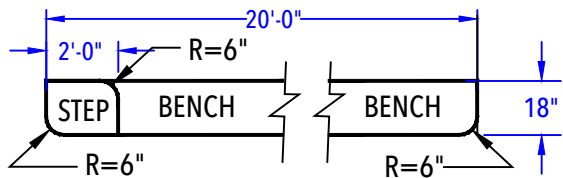
OFFSET BENCH & STEP OUT DETAIL (After Concrete & Liner) N.T.S.
