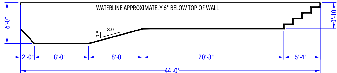
DEPTH DETAIL
