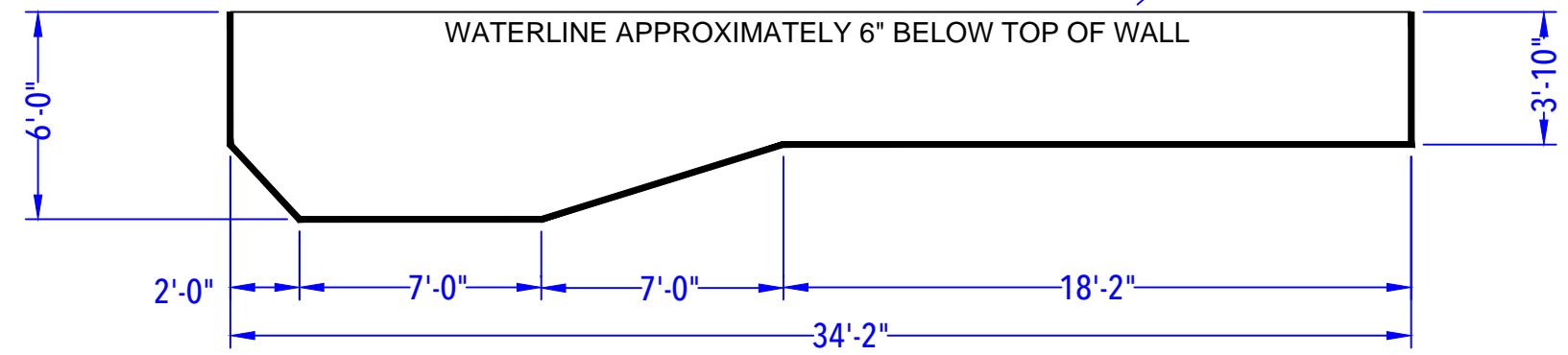
DEPTH DETAIL
