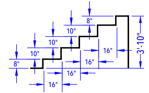
STEP DETAIL (After Bottom & Liner) N.T.S.
