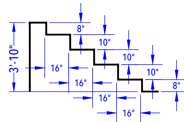
ENTRY STEP DETAIL (After Bottom & Liner) N.T.S.
