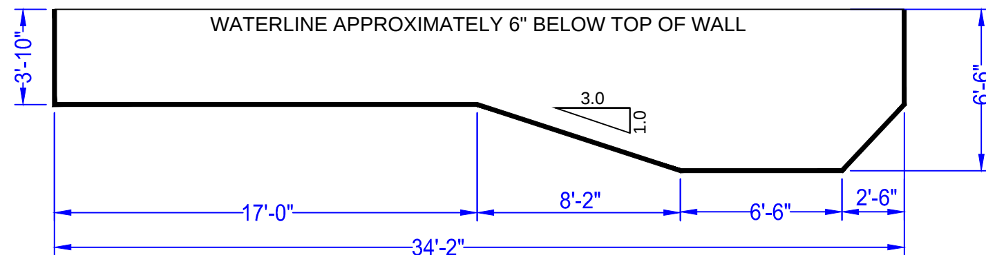
DEPTH DETAIL
