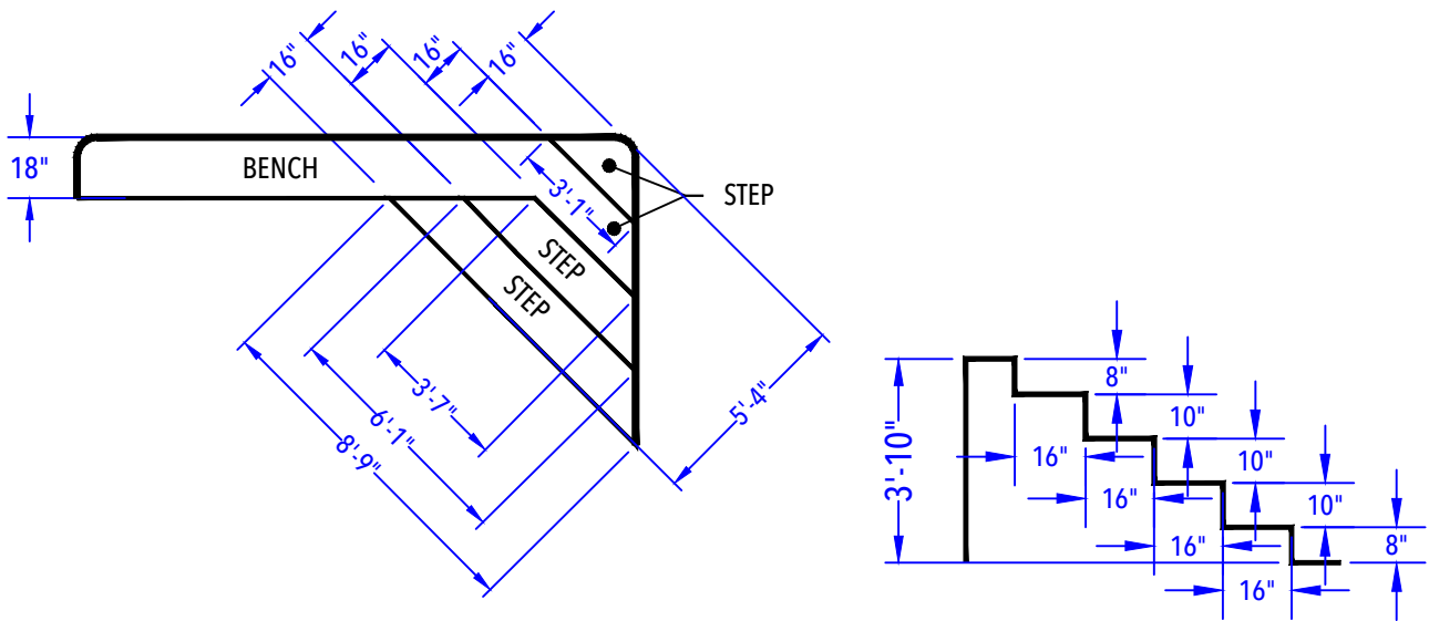
ENTRY STEP DETAIL (After Concrete & Liner) N.T.S.
