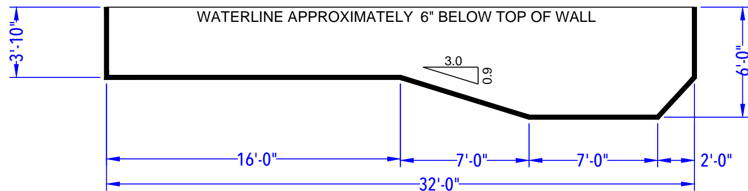
DEPTH DETAIL
