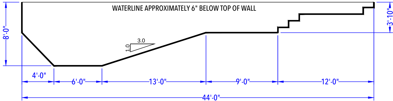
DEPTH DETAIL
