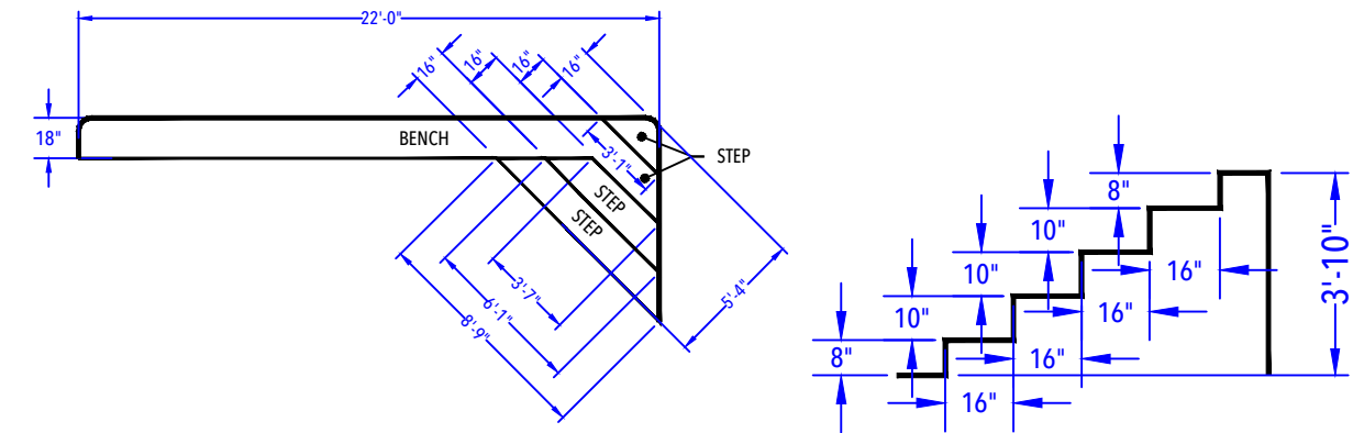
ENTRY STEP DETAIL (After Concrete & Liner) N.T.S.
