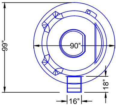
SPILOVER SPA DETAIL (After Concrete & Liner) N.T.S.
