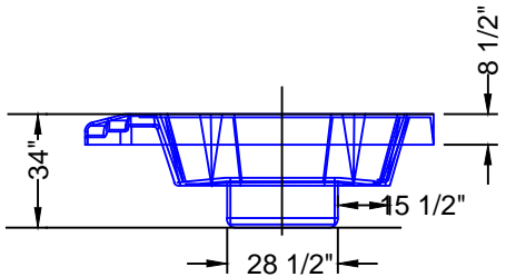
ENTRY STEP DETAIL (After Concrete & Liner) N.T.S.
