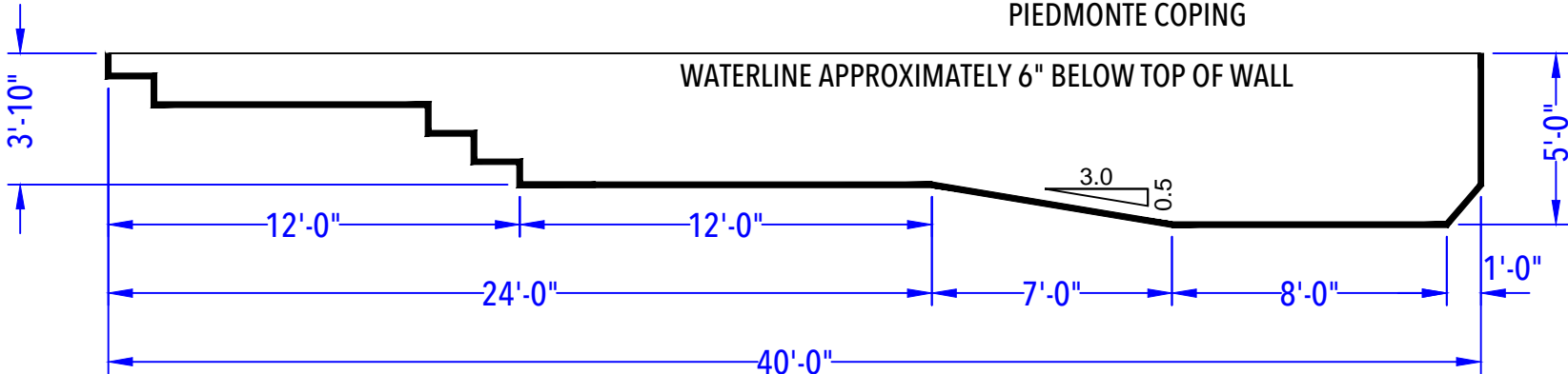
DEPTH DETAIL
