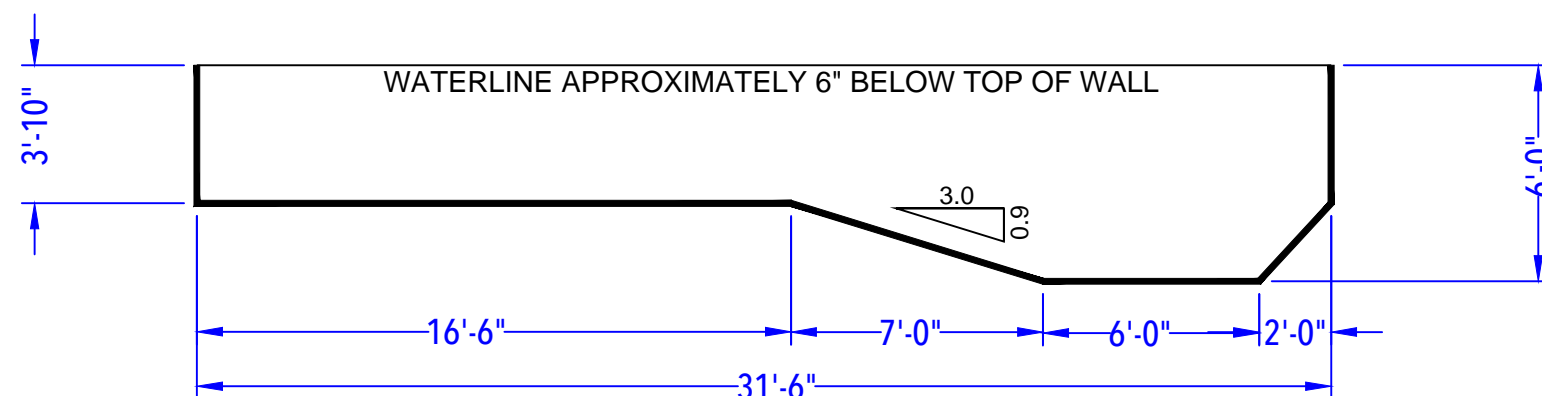
DEPTH DETAIL
