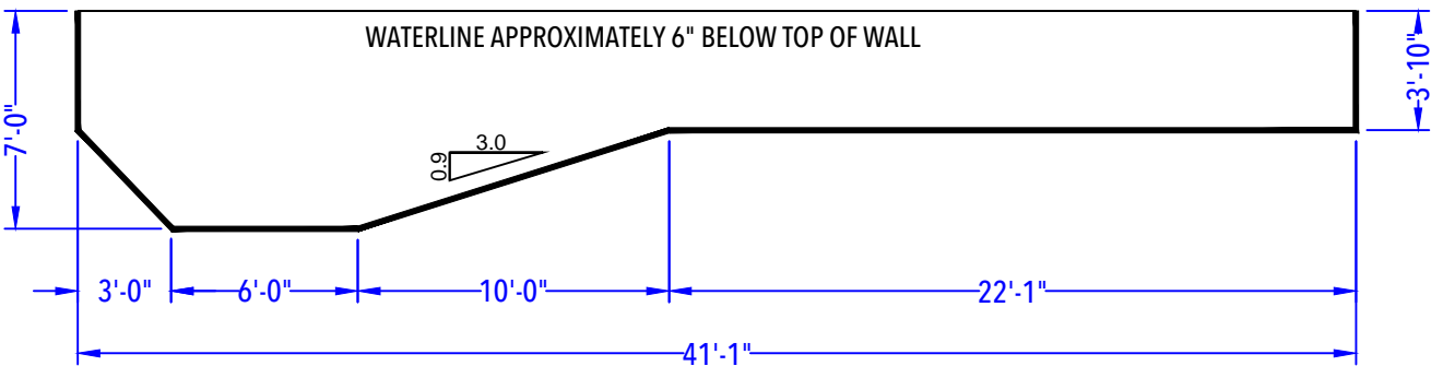
DEPTH DETAIL
