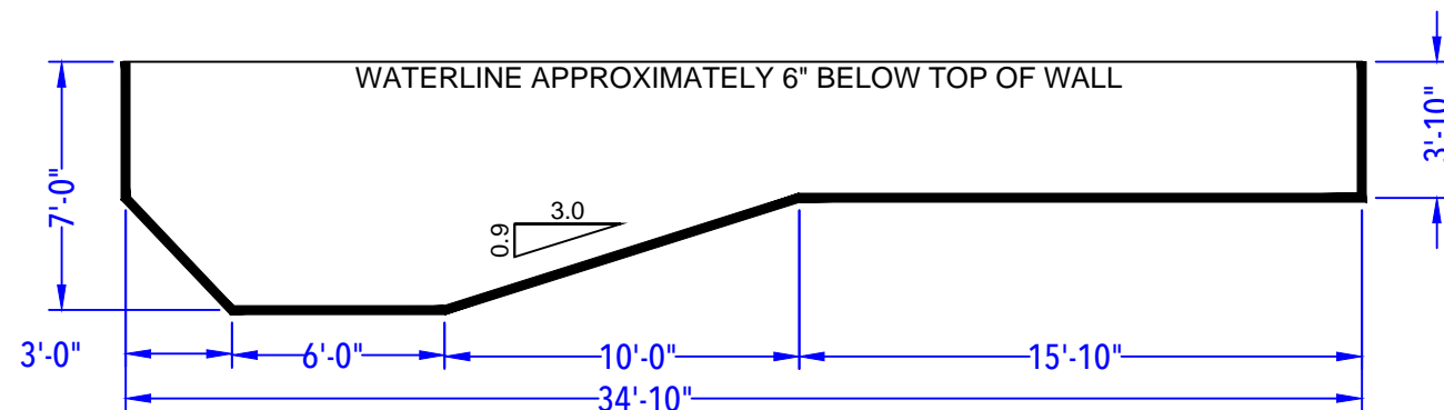
DEPTH DETAIL
