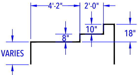
DEEP END BENCH & STEP OUT DETAIL (After Concrete & Liner) N.T.S.
