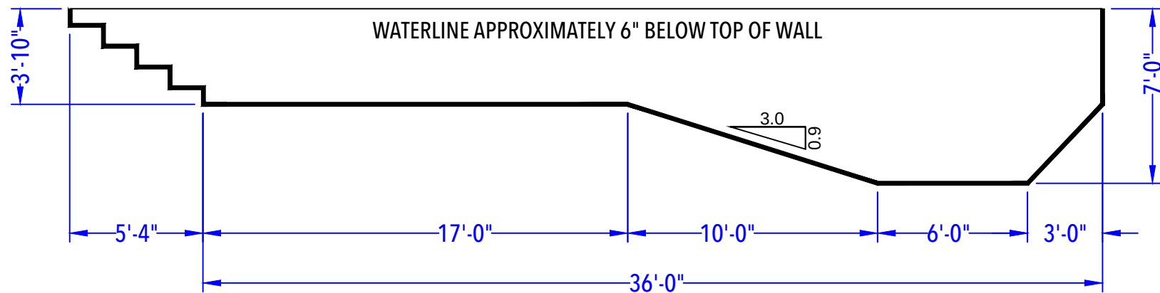
DEPTH DETAIL
