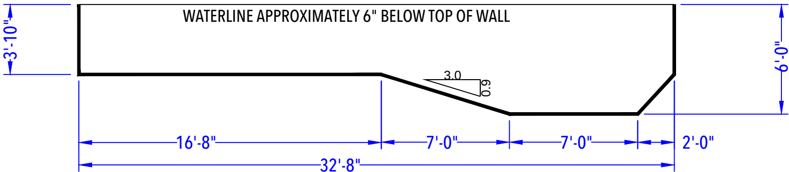
DEPTH DETAIL
