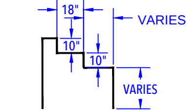
DEEP END BENCH & STEP OUT DETAIL (After Concrete & Liner) N.T.S.
