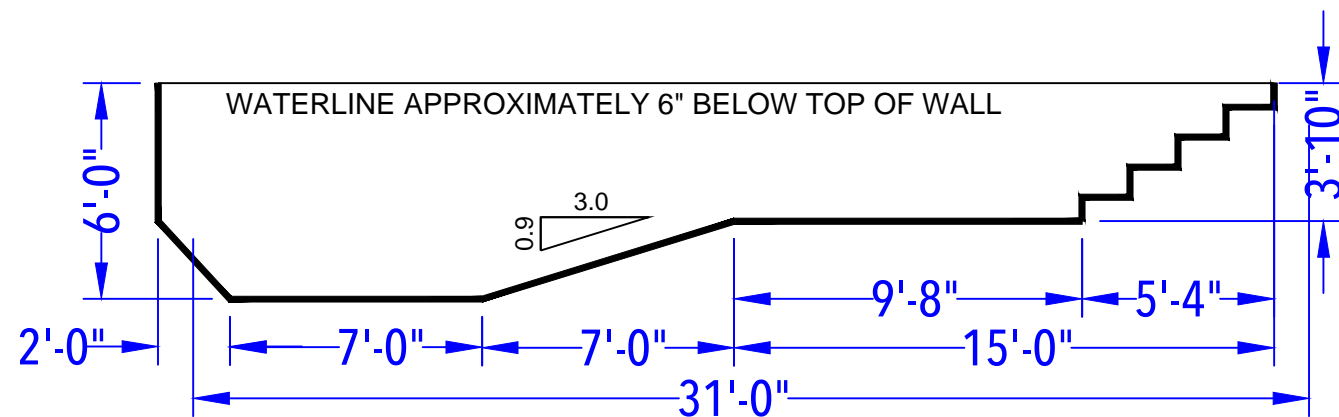
DEPTH DETAIL
