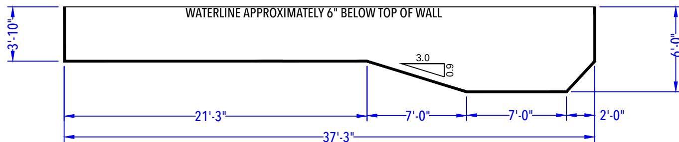
DEPTH DETAIL
